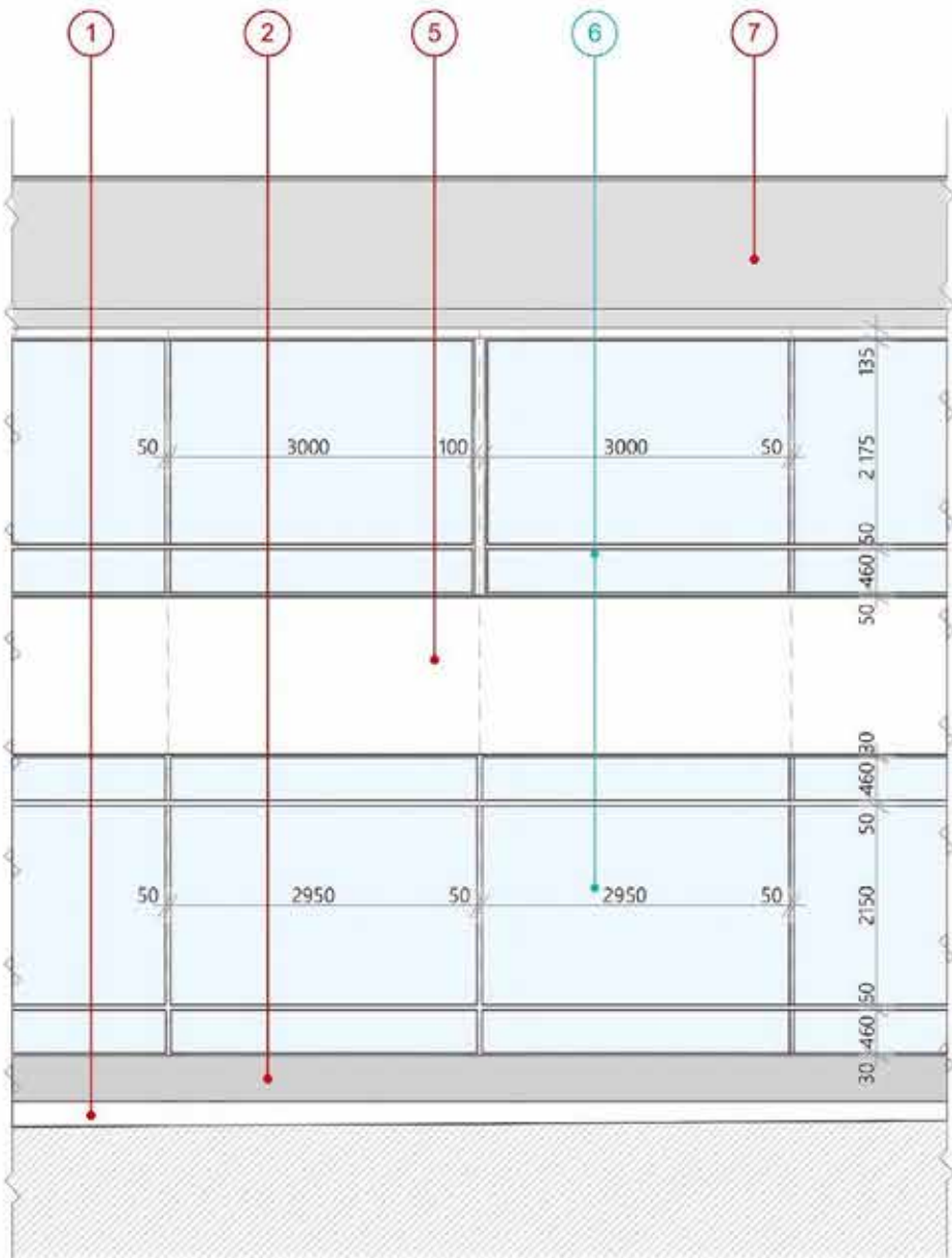
Fragment de la facade principal (1:100)
